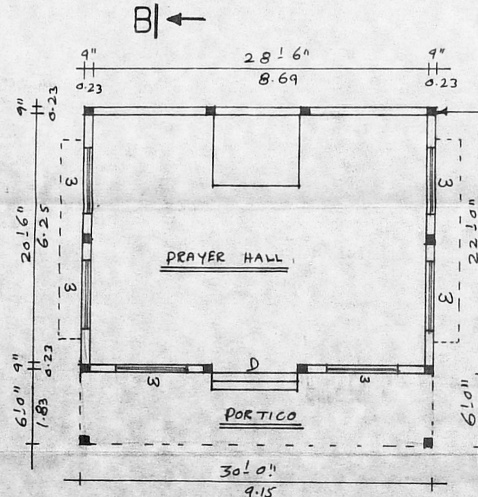
PLAN
